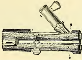
Mechanism of Needham's Needle Gun.
